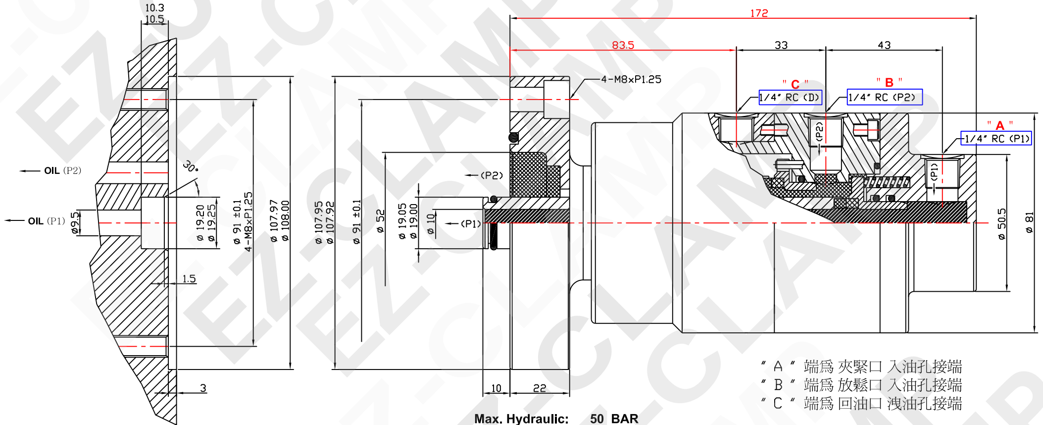
ROTOR HOUSING
