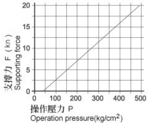
SP-32B 油壓頂出型 Hydraulic extended piston rod
