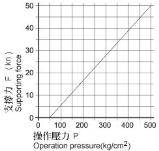
SP-40B 油壓頂出型 Hydraulic extended piston rod
