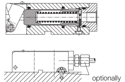
Low-block clamping cylinder with locking piston (page 4)
