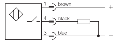
pnp (+) switching
